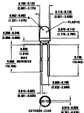
Package E
