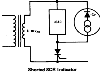
Shorted SCR Indicator
