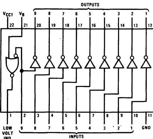
Dual-In-Line Package
