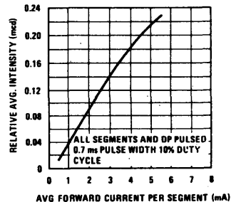
Average Light Intensity vs Average Forward Current
