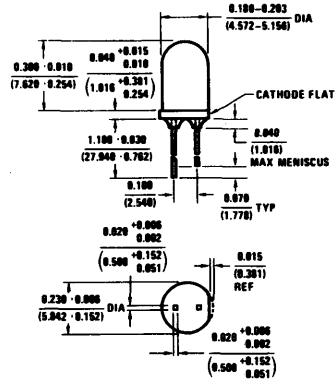
Package B
