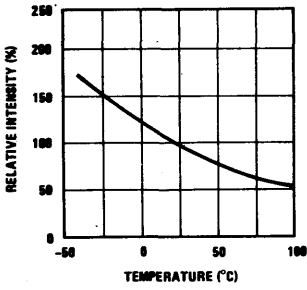
Light Intensity vs Ambient Temperature
