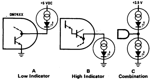
FIGURE 7. TTL Indicators
