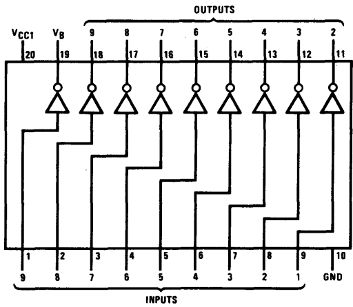
Dual-In-Line Package
