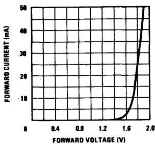
Forward Current ( I_F ) vs Forward Voltage ( V_F )
