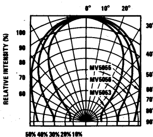
FIGURE 5. Spatial Distribution
