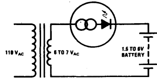
Small Battery Trickle Charger
