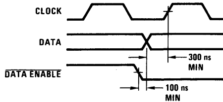
FIGURE 4. Timing Relationships
