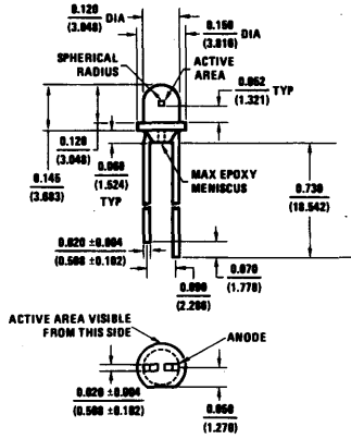
Package G
