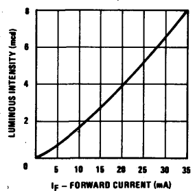
FIGURE 9. Luminous Intensity vs Forward Current
