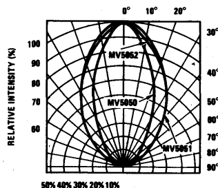
FIGURE 6. Spatial Distribution
