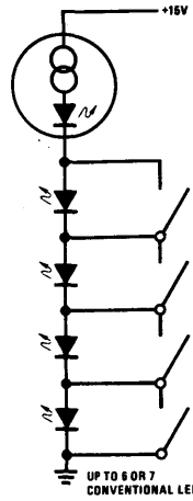
UP TO 6 OR 7 CONVENTIONAL LEDS Switch or Circuit Breaker or Relay Closure Indicator
