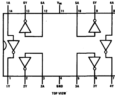
DS75492 Dual-In-Line Package
