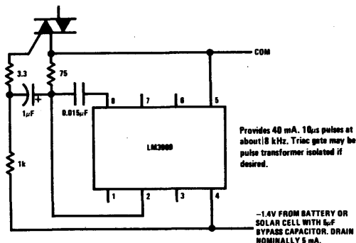
Triac Trigger
