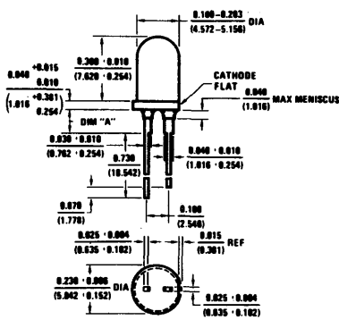
Package A
