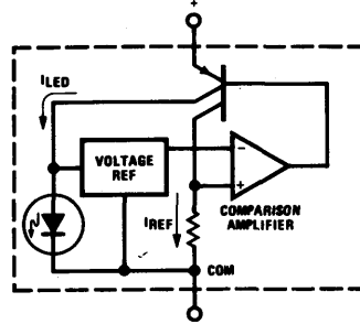
FIGURE 2. Simplified Schematic
