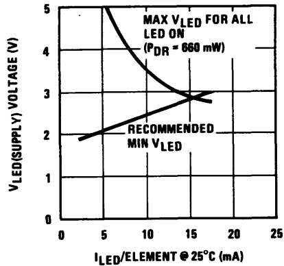
FIGURE 3. LED Supply Voltage Range
