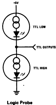
Logic Probe
