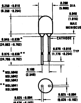
Package C
